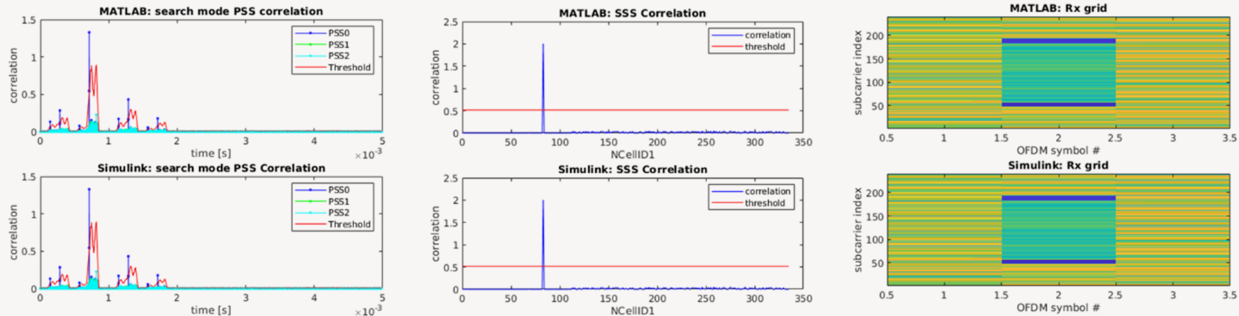
Plots comparing the Simulink implementation vs. the MATLAB algorithm for PSS detection, SSS detection, and the grid for the decoded signal.
