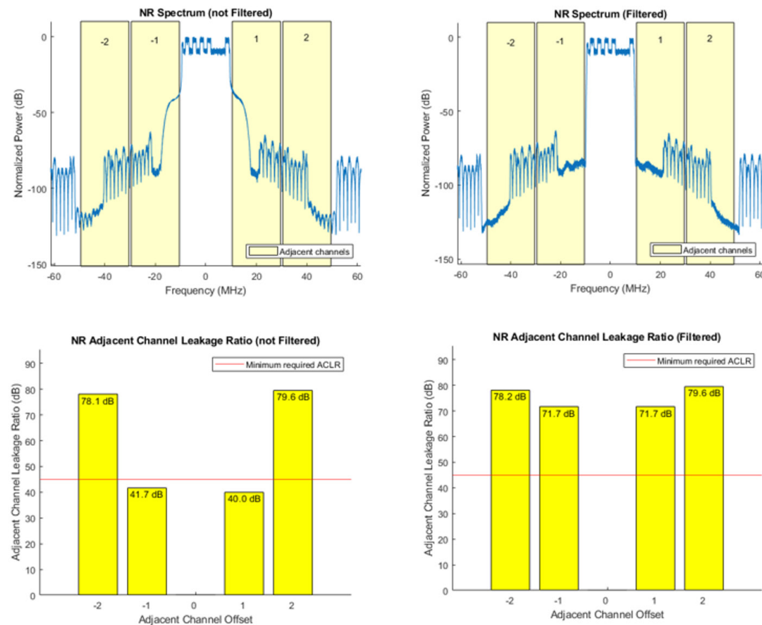
Measuring the impact of filtering on an NR-TM waveform.
