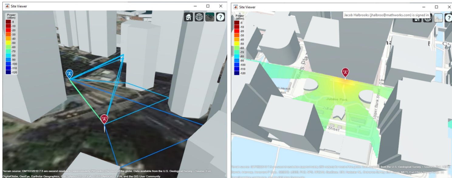
Visualization of propagation paths between points (left) and cellular signal coverage (right) on street maps.
