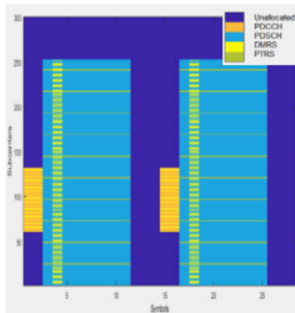
5G Resource Grid
