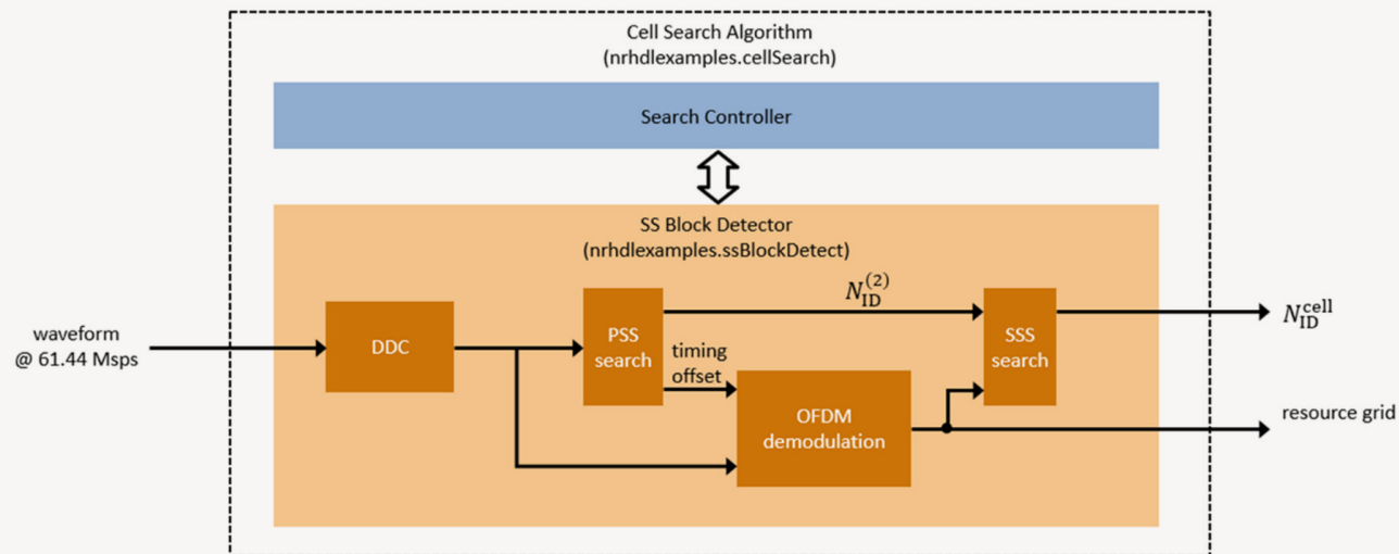
Hardware-software partitioning of the 5G NR HDL Cell Search algorithm. The SS Block Detector will be deployed to hardware, while the Search Controller will be deployed to software.
