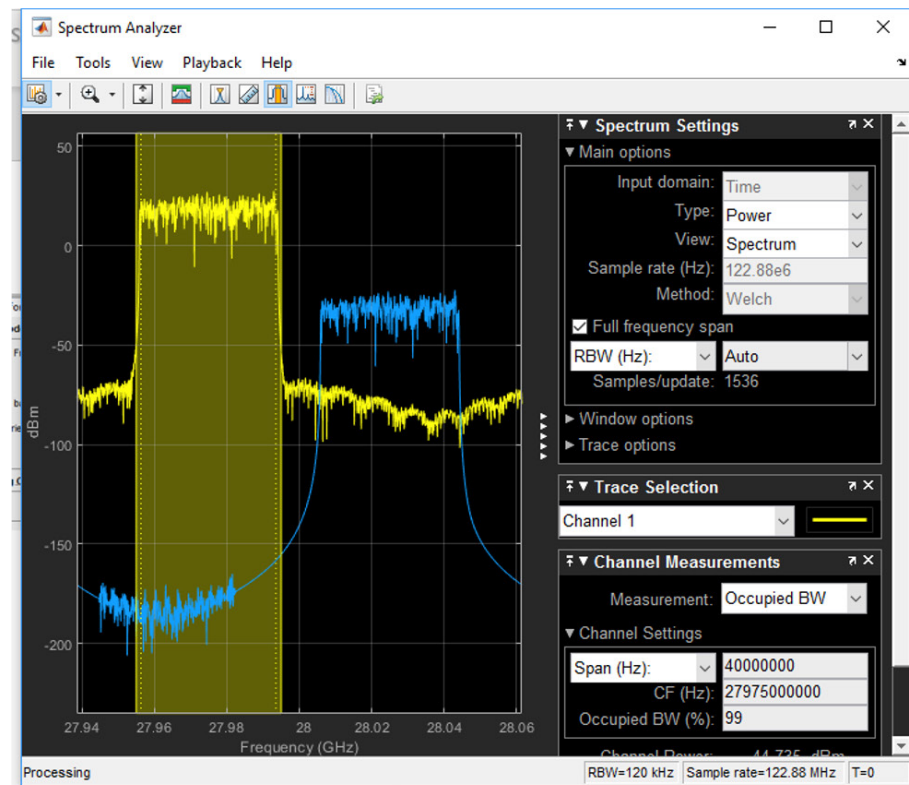
Generation (left) and analysis (right) of a 5G NR test model (NR-TM) waveform.
