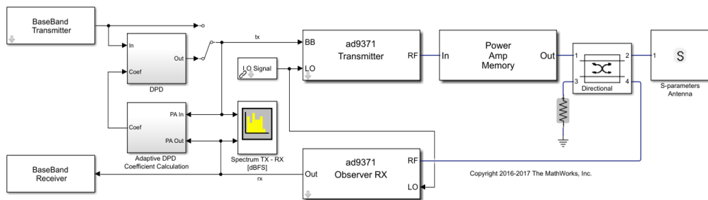
Closed-loop transceiver model with power amplifier and adaptive DPD algorithm. The lab-validated AD9371 models include real-life effects. The Volterra series model of the power amplifier includes non-linearity and memory effects. The loop simulation includes low and high-power effects, timing, and frequency selectivity over the signal bandwidth. The adaptive DPD algorithm improves the device linearity within the signal bandwidth.
