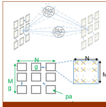
3GPP 38.901 Channel Model
