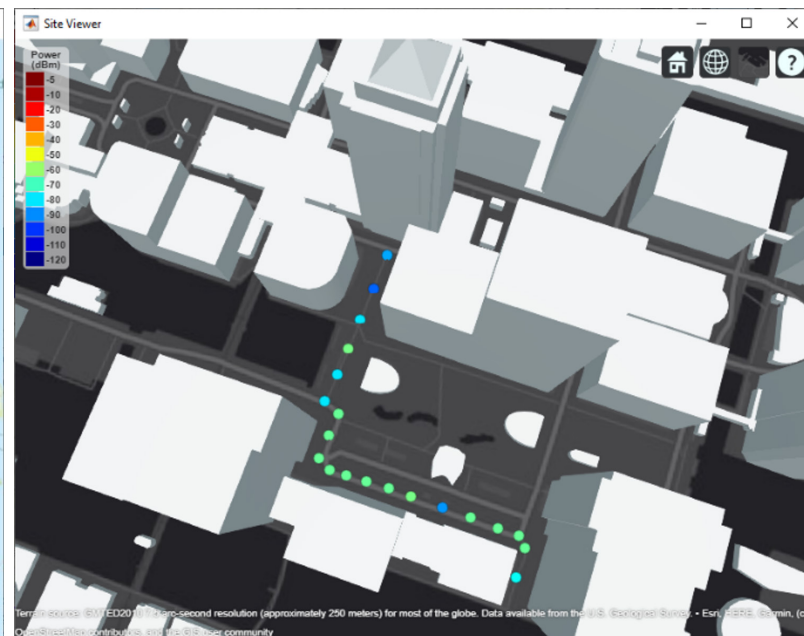
Visualization of data throughput capacity (left) and drive test measurements (right) on street maps.
