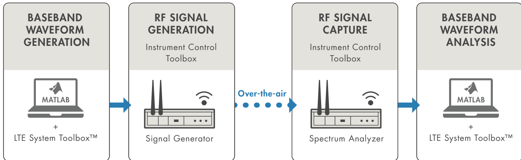
Over-the-air testing with MATLAB and test and measurement instruments.
