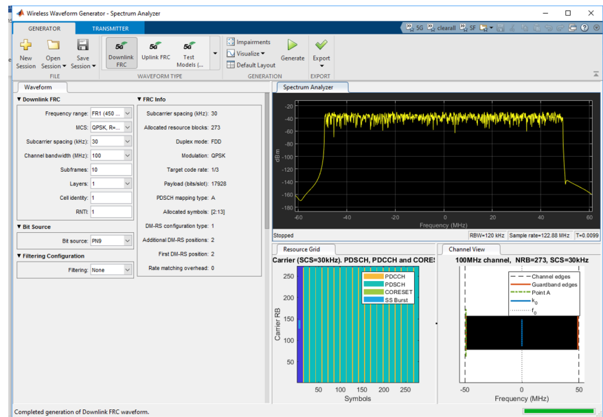
Using the 5G Waveform Generator to generate a 100 MHz fixed reference channel (FRC) with 30 kHz spacing according to TS 38.101-1.
